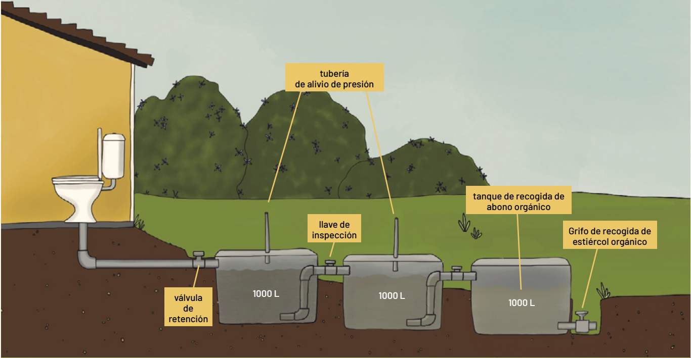
Tanque biodigestor
